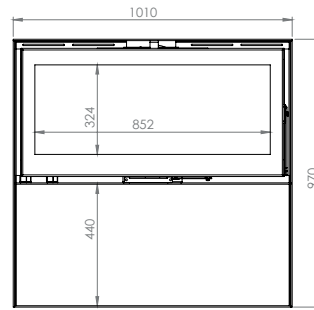
MODUL-ART 16/9 woodbox
