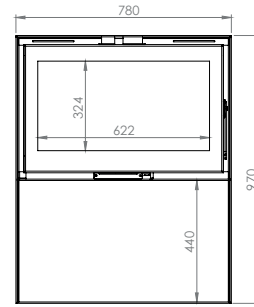
MODUL-ART 77 woodbox
