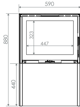
MODUL-ART 58 woodbox
